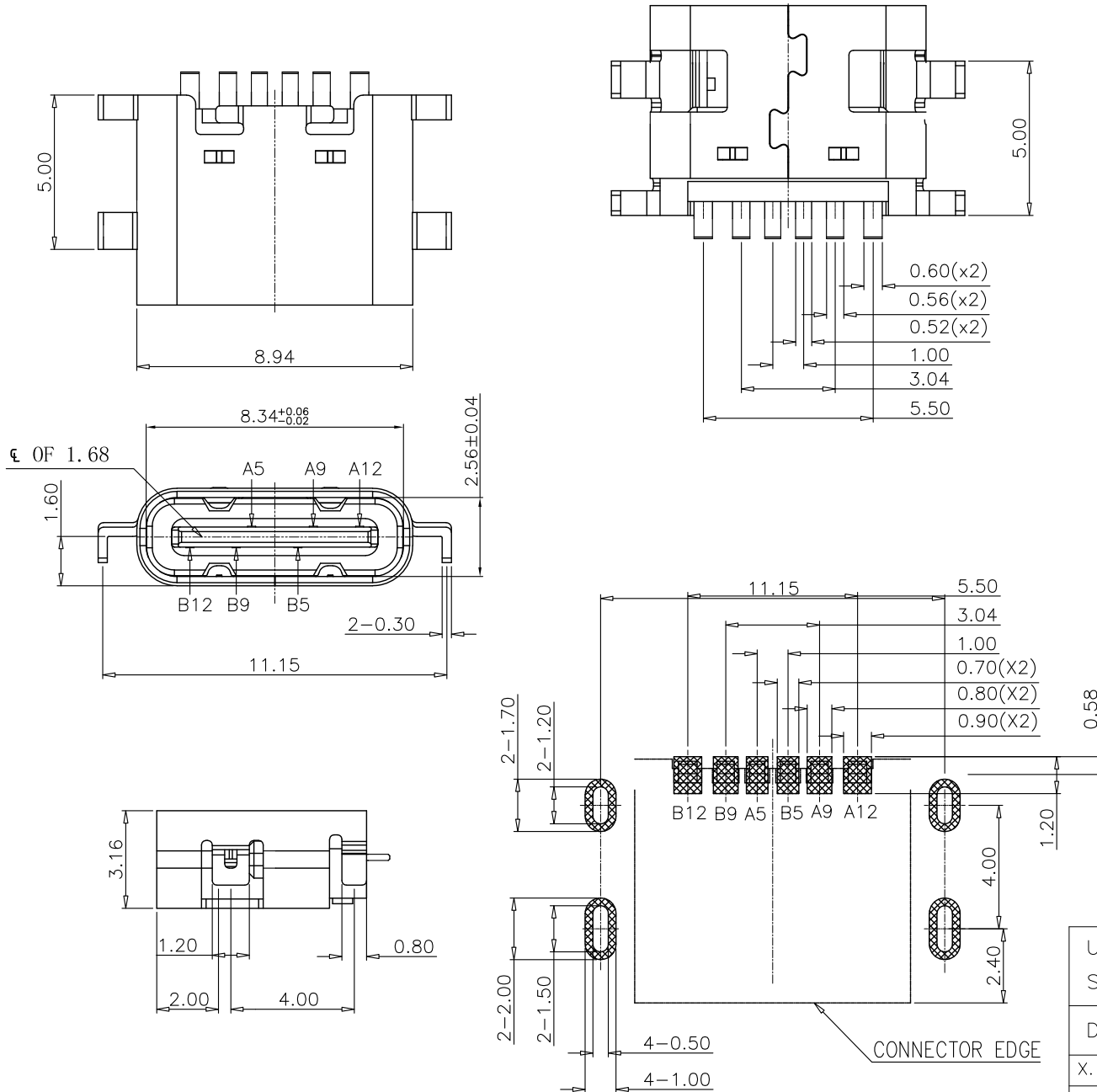
RECOMMENDED PCB LAYOUT(TOP VIEW) THICKNESS 1.6±0.10MM;DEFAULT TOLERANCE:±0.05
