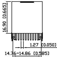
RECOMMENDED PLUG DIMENSION:
