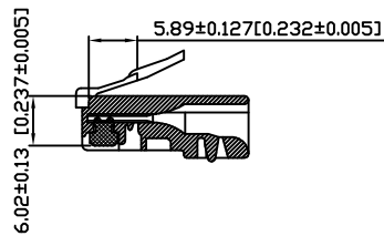
RECOMMENDED PLUG DIMENSION:
