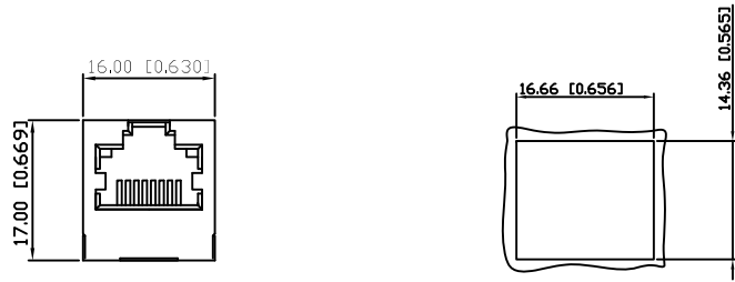
RECOMMENDED PANEL CUTOUT DIMENSION
