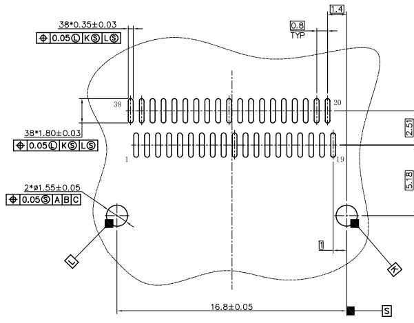
PCB LAYOUT
