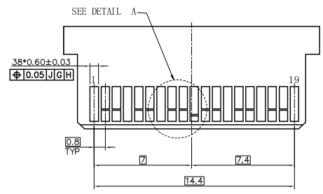
QSFP14 MODULE CARD
