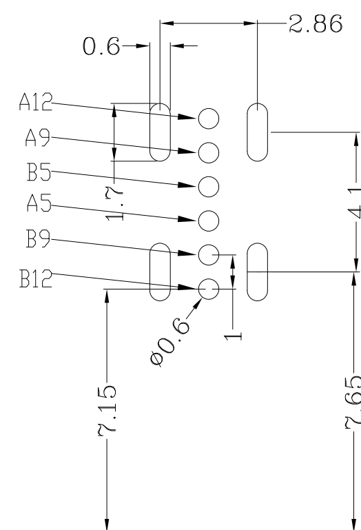
RECOMMENDED P.C.B. LAYOUT TOLERANCE UNSPECIFIED \pm 0.05\text{mm}
