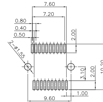
DETAIL A(SCALE 2:1)
