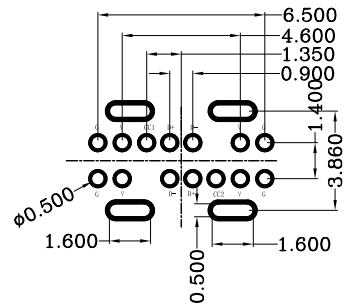
RECOMMENDED P.C.B. LAYOUT TOLERANCE UNSPECIFIED ±0.05mm
